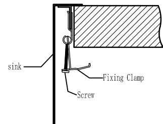
TOPMOUNT INSTALLATION
