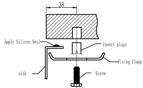
UNDERMOUNT INSTALLATION
