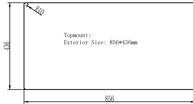
TOPMOUNT INSTALLATION
