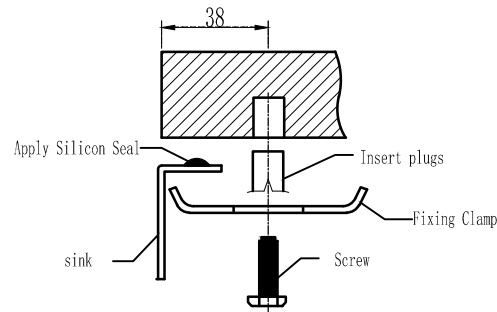
UNDERMOUNT INSTALLATION
