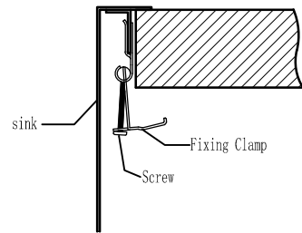
TOPMOUNT INSTALLATION
