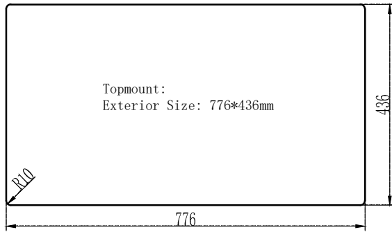
Topmount Installation
