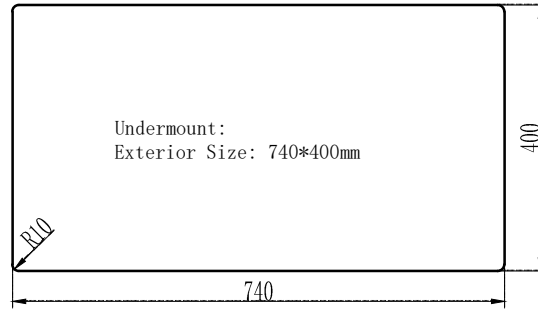
Undermount Installation
